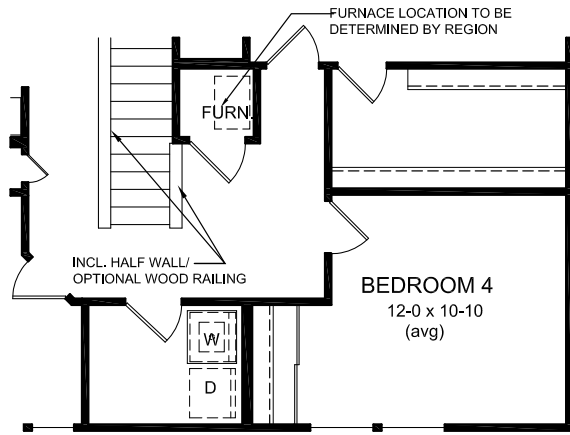
ALTERNATE SECOND FLOOR DESIGN w/ OPT. BEDROOM 4
