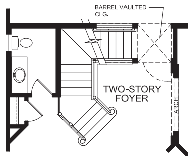
OPT. OPEN BASEMENT STAIR
