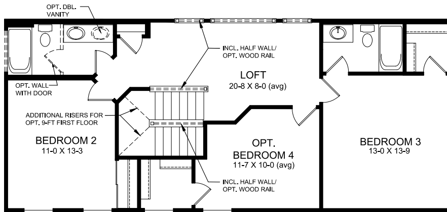
SECOND FLOOR DESIGN SHOWN w/ OPT. BEDROOM 4 & OPT. BEDROOM 3 BATH
