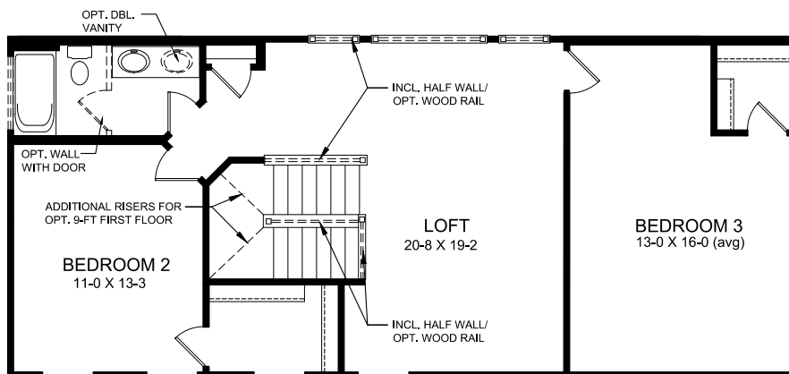
SECOND FLOOR DESIGN
