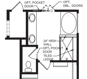
OPTIONAL DELUXE GARDEN BATH
