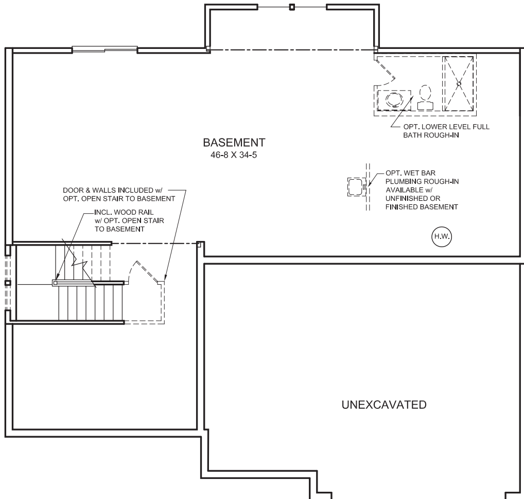
OPTIONAL WALKOUT BASEMENT w/ REAR FRAME WALL
