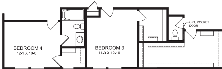
OPTIONAL BEDROOM 4 BATH w/ OPTIONAL FIRST FLOOR LAUNDRY ROOM
