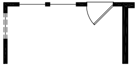
OPT. DOOR AND WINDOWS W/ EXPANDED MORNING ROOM
