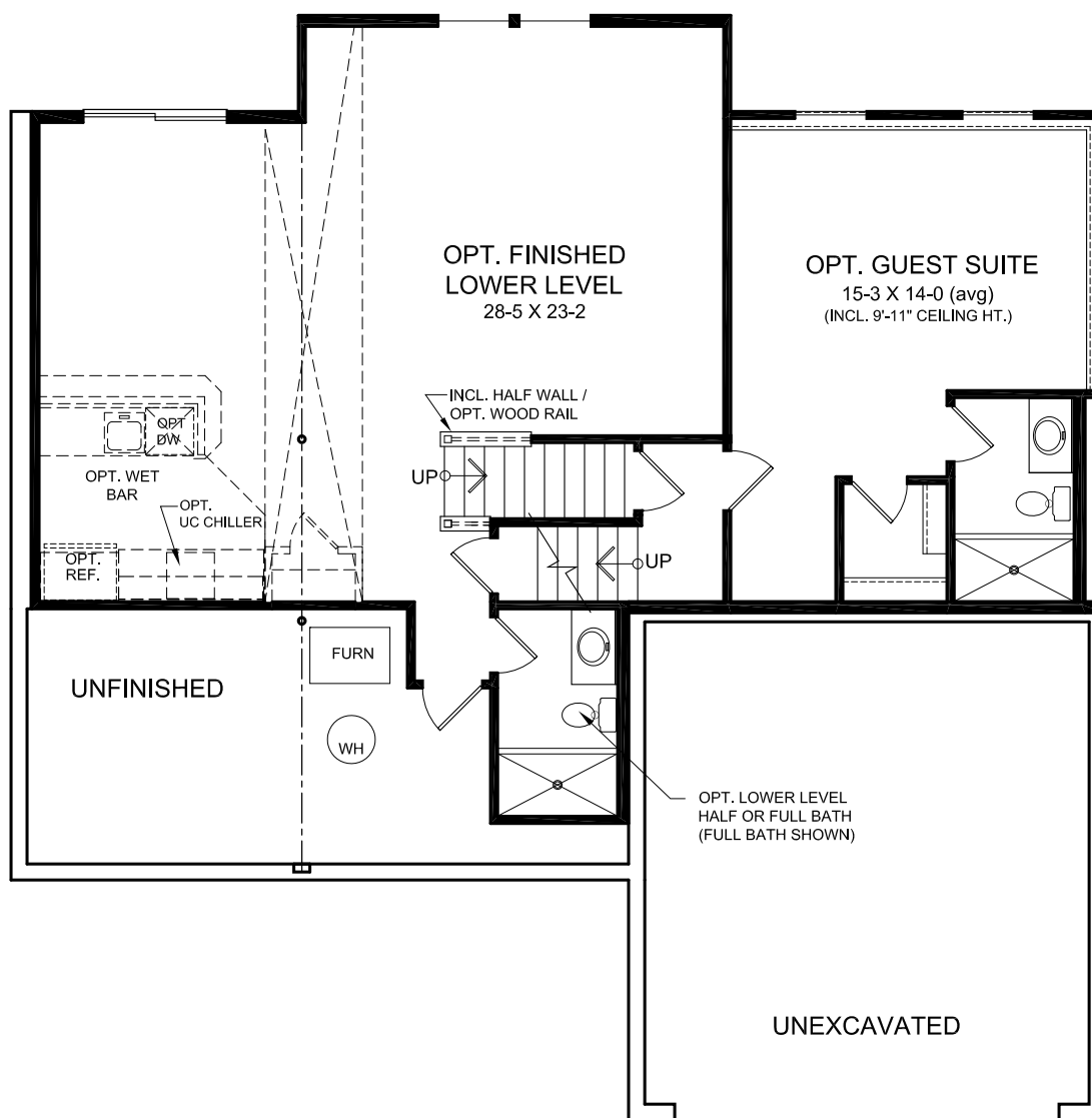
OPTIONAL WALKOUT FINISHED LOWER LEVEL w/ REAR FRAME WALL
