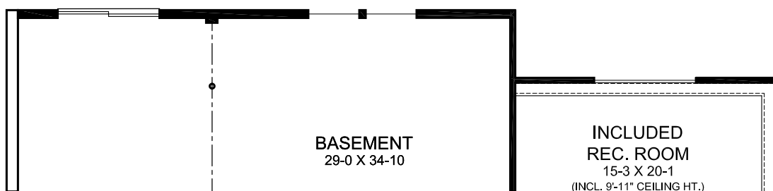
OPTIONAL WALKOUT BASEMENT w/ REAR FRAME WALL
