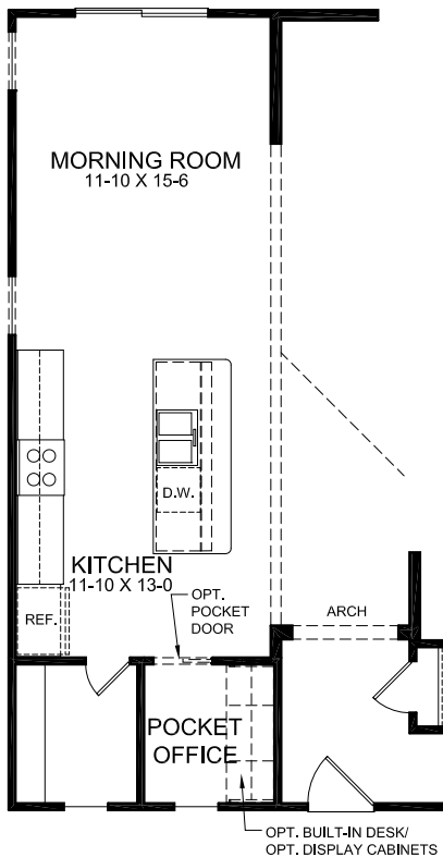
OPT. EXPANDED MORNING ROOM ADDS APPROX. 47 SQ. FT.
