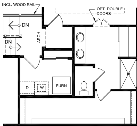
PARTIAL UPPER LEVEL DESIGN STANDARD PLAN
