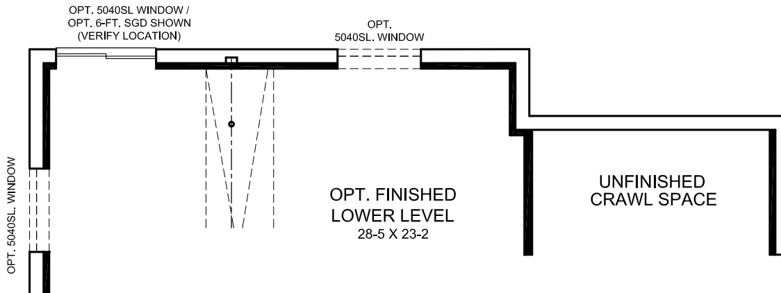
OPTIONAL FINISHED LOWER LEVEL DESIGN INCLUDED 8-FT BASEMENT CLG. HEIGHT w/ OPTIONAL EXPANDED MORNING ROOM
