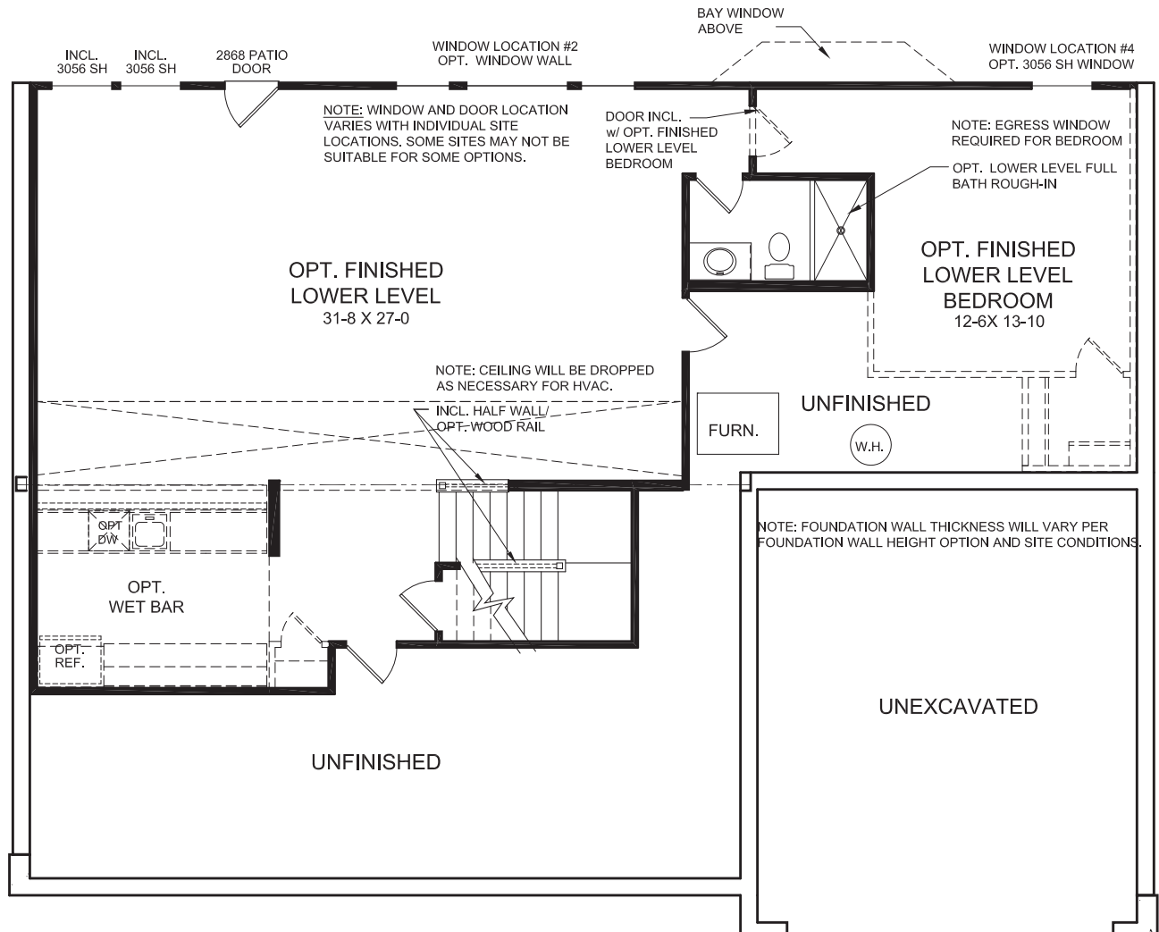
OPTIONAL WALKOUT FINISHED LOWER LEVEL DESIGN (ATLANTA ONLY)
