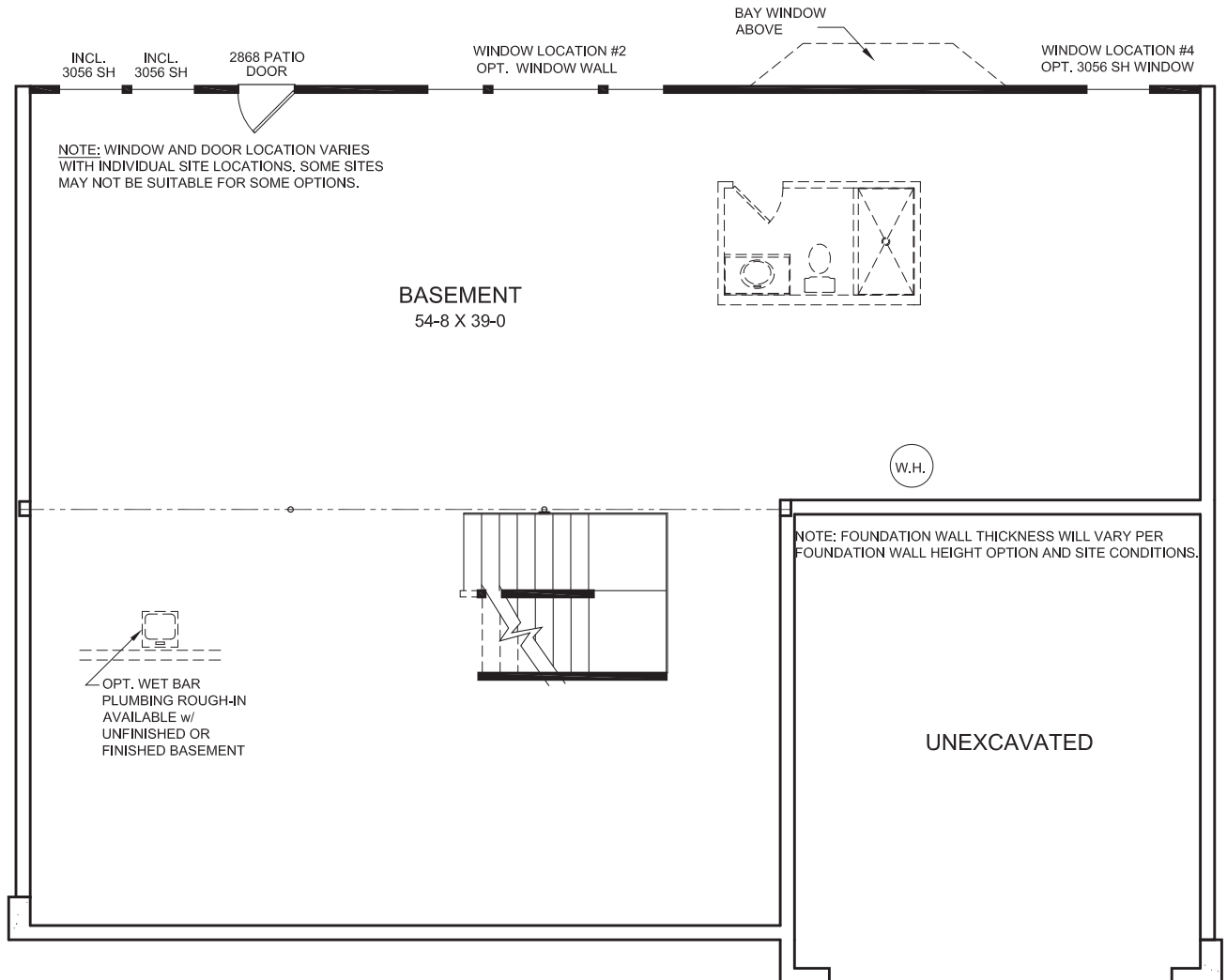
OPTIONAL WALKOUT BASEMENT DESIGN (ATLANTA ONLY)
