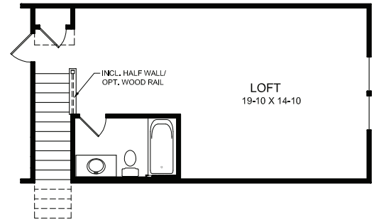
OPTIONAL LOFT PARTIAL PLAN DESIGN w/ OPT. BEDROOM & FULL BATH (SHOWN w/ OPT. BASEMENT)
