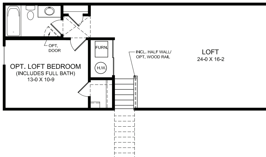
OPTIONAL LOFT DESIGN w/ OPTIONAL BEDROOM & FULL BATH
