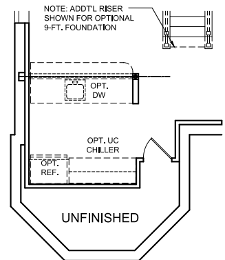
OPTIONAL WET BAR ADDS ADDITIONAL 94 SQ. FT. (FOR AMERICAN CLASSIC AND NANTUCKET RETREAT EXTERIORS ONLY)
