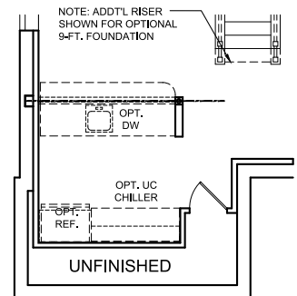
OPTIONAL WET BAR ADDS ADDITIONAL 94 SQ. FT. (FOR PACIFIC CRAFTSMAN AND VILLA TUSCANO EXTERIORS ONLY)
