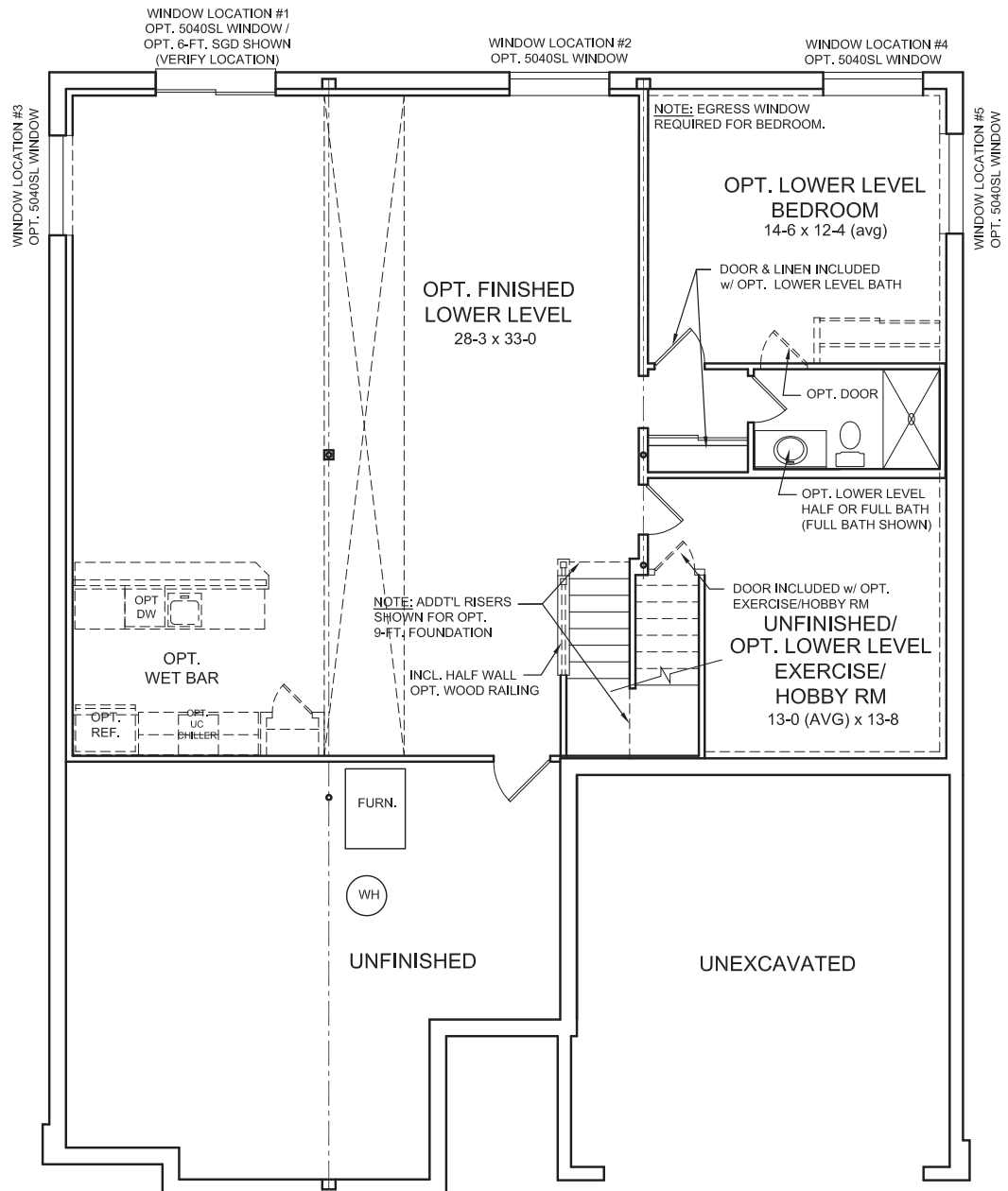
OPTIONAL FINISHED LOWER LEVEL DESIGN INCLUDED 8-FT BASEMENT CLG. HEIGHT
