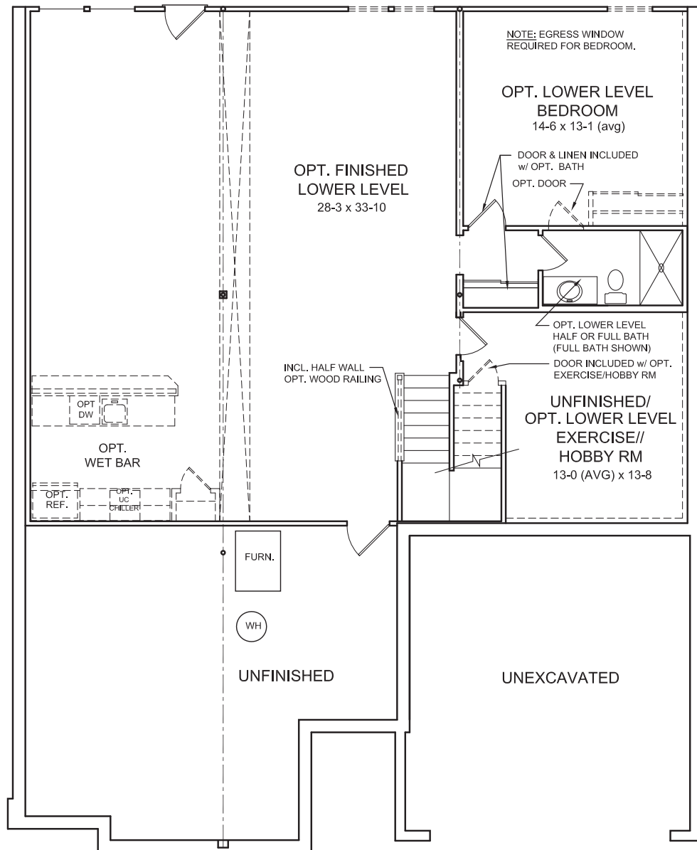
OPTIONAL WALKOUT FINISHED LOWER LEVEL DESIGN (ATLANTA ONLY) w/ INCL. REAR FRAME WALL INCLUDED 9-FT BASEMENT CLG. HEIGHT
