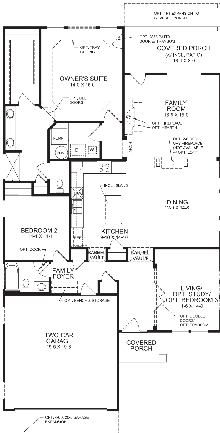
FIRST FLOOR DESIGN (INCLUDES 9 FT FIRST FLOOR CEILING HEIGHT)
