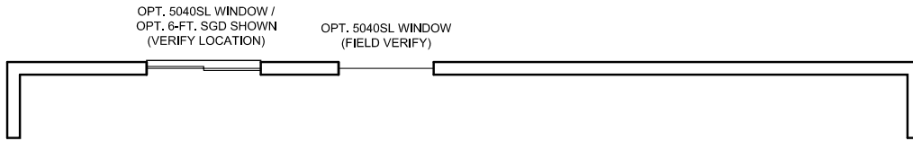
OPTIONAL BASEMENT DESIGN w/ OPT. SLIDING GLASS DOOR
