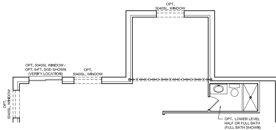
OPTIONAL FINISHED LOWER LEVEL DESIGN w/ OPT. SUNROOM
