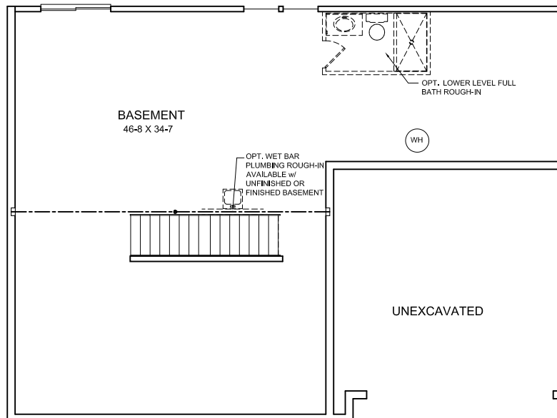
OPTIONAL WALKOUT BASEMENT w/ REAR FRAME WALL
