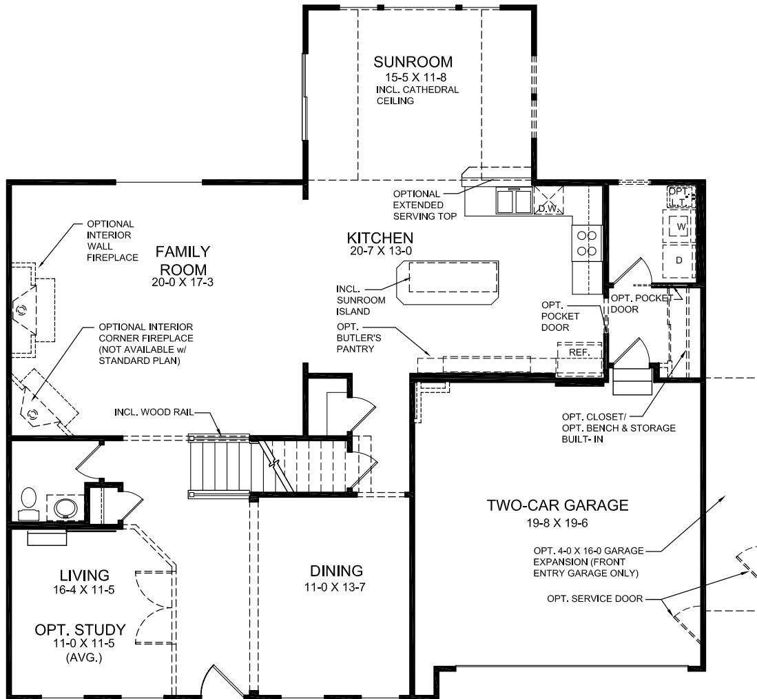
ALTERNATE FIRST FLOOR DESIGN w/ SUNROOM & INCL. GOURMET ISLAND
