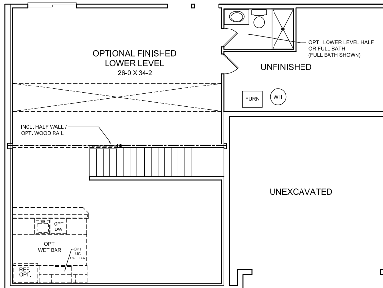
OPTIONAL WALKOUT FINISHED LOWER LEVEL w/ REAR FRAME WALL
