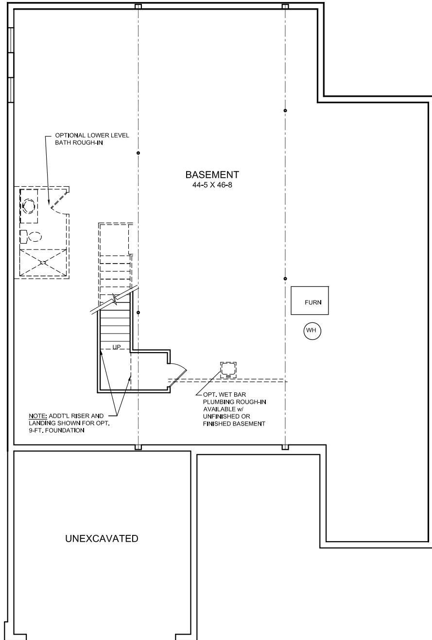
OPTIONAL BASEMENT DESIGN w/ OPT. LOFT
