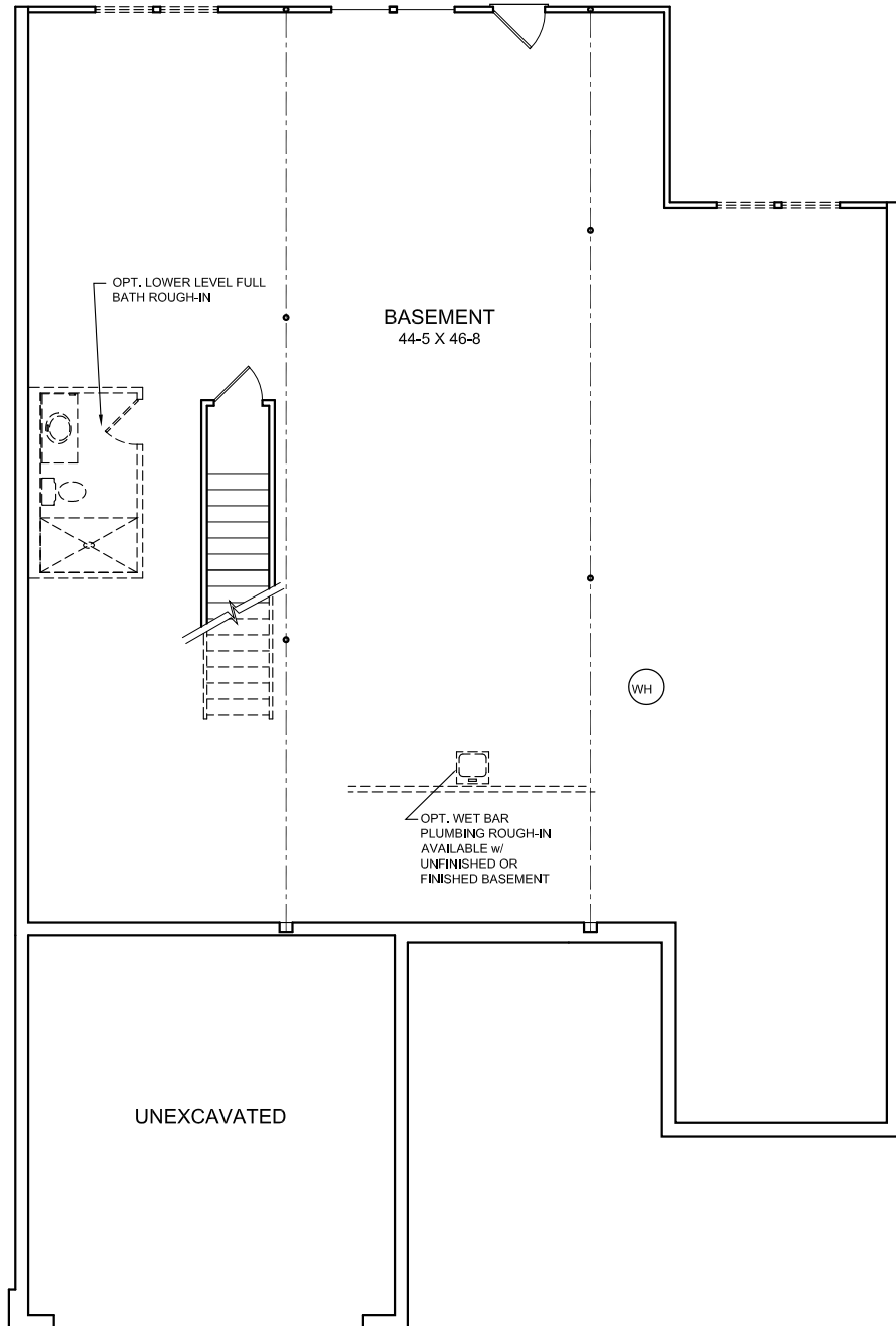
OPTIONAL WALKOUT BASEMENT DESIGN (ATLANTA ONLY) w/ INCL. REAR FRAME WALL INCLUDED 9-FT BASEMENT CLG. HEIGHT
