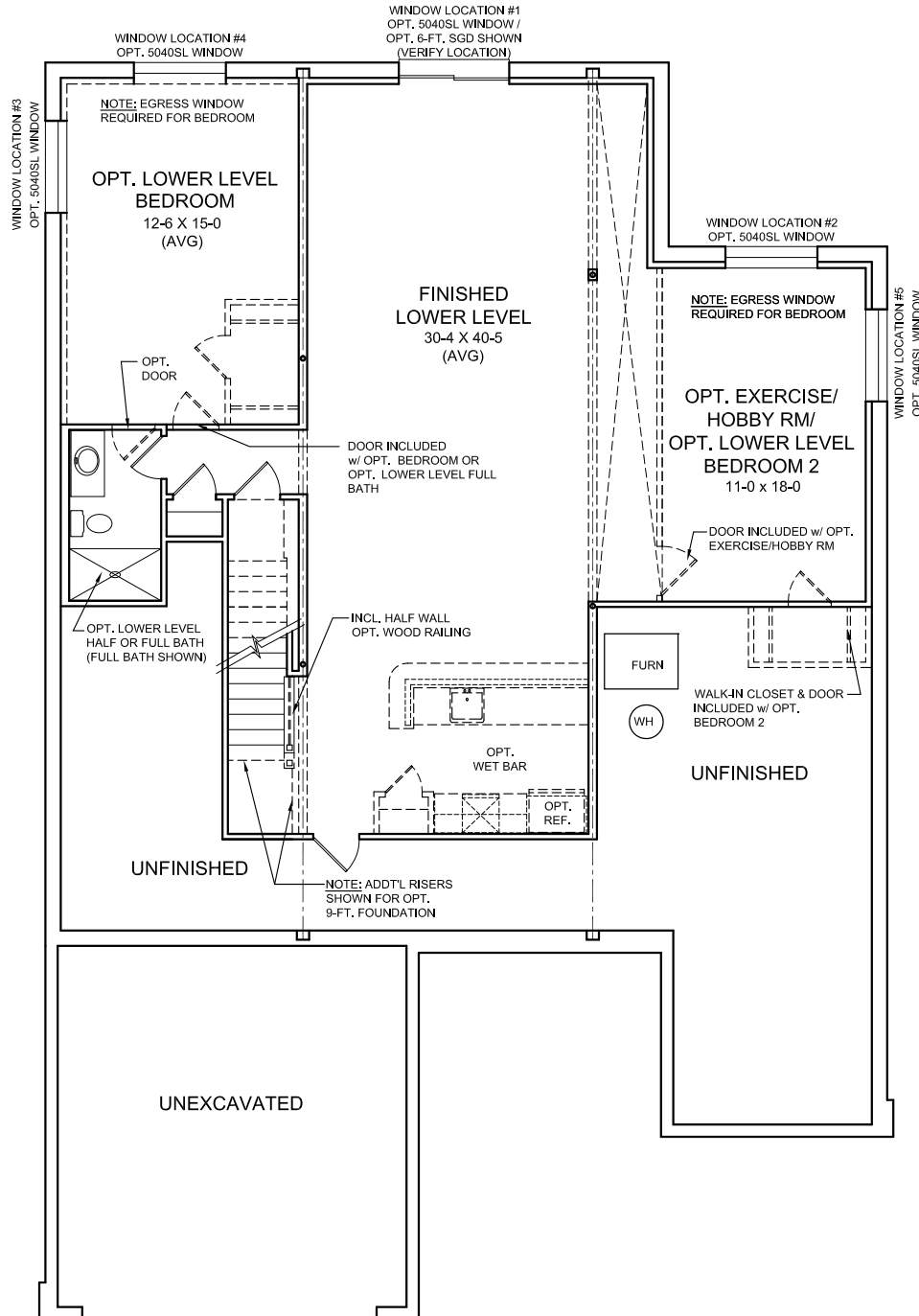
OPTIONAL FINISHED LOWER LEVEL DESIGN w/ OPT. LOFT
