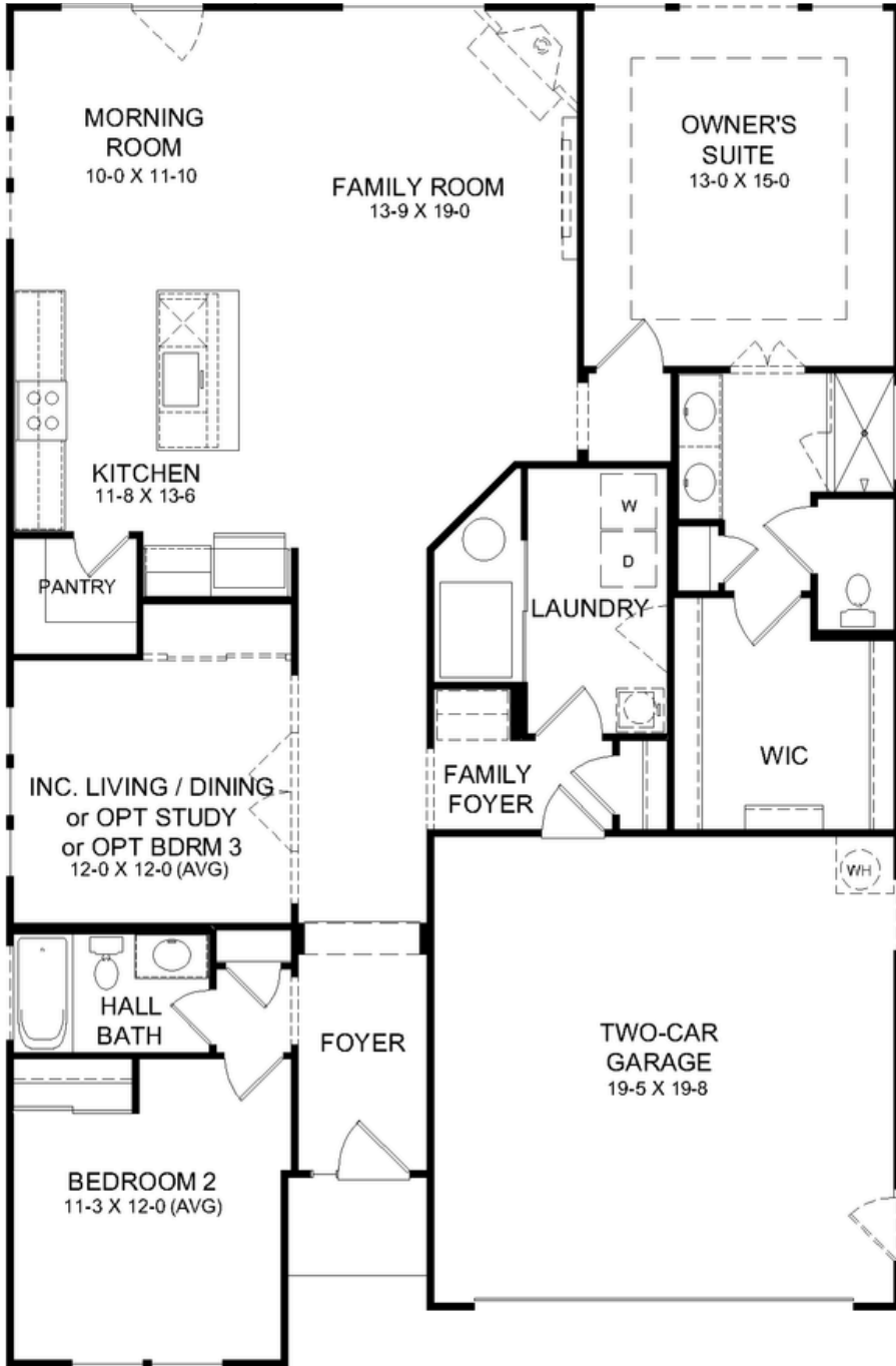
FIRST FLOOR DESIGN
