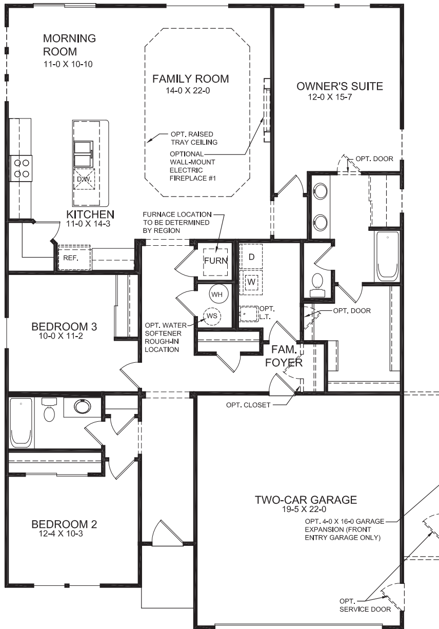
FIRST FLOOR DESIGN (STANDARD PLAN)
