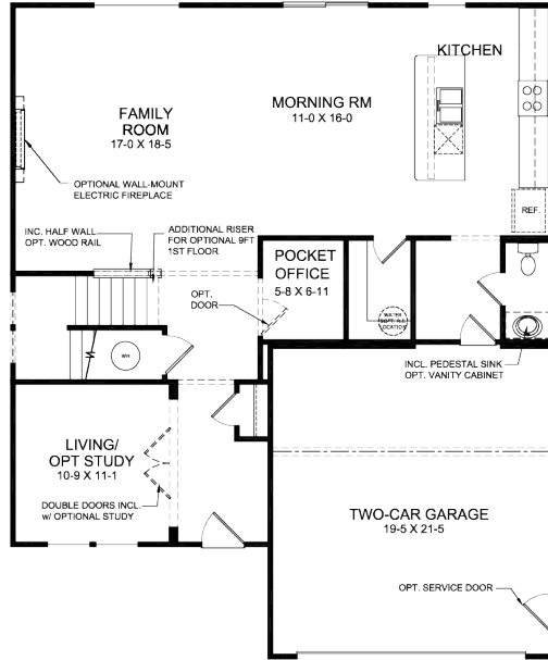
FIRST FLOOR DESIGN (STANDARD PLAN)
