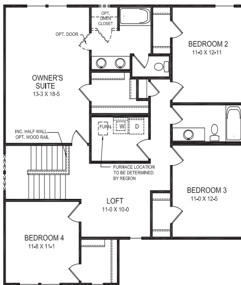
SECOND FLOOR DESIGN
