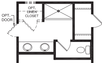
OPT. 5-FT SHOWER IN LIEU OF INCLUDED TUB
