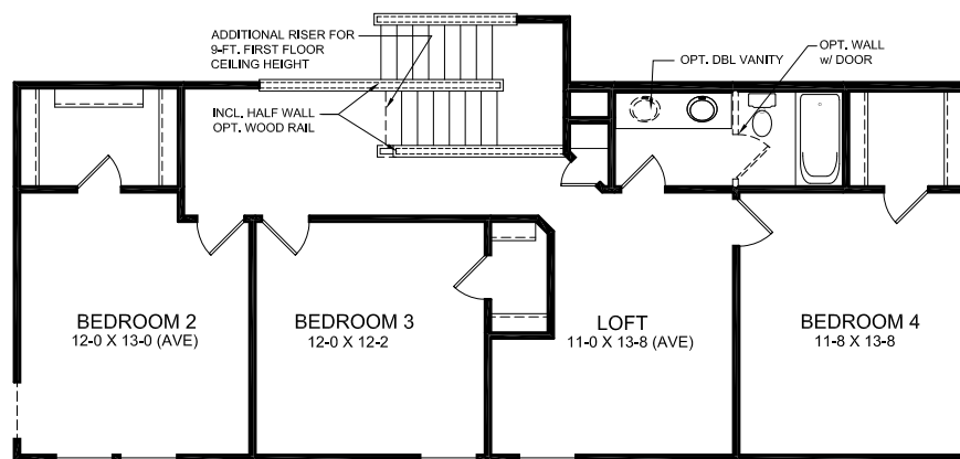
SECOND FLOOR DESIGN
