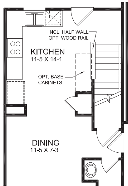
FIRST FLOOR DESIGN A OPT. STANDARD PLAN
