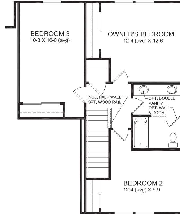
ALTERNATE SECOND FLOOR DESIGN B
