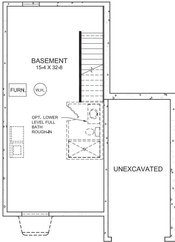
BASEMENT DESIGN A
