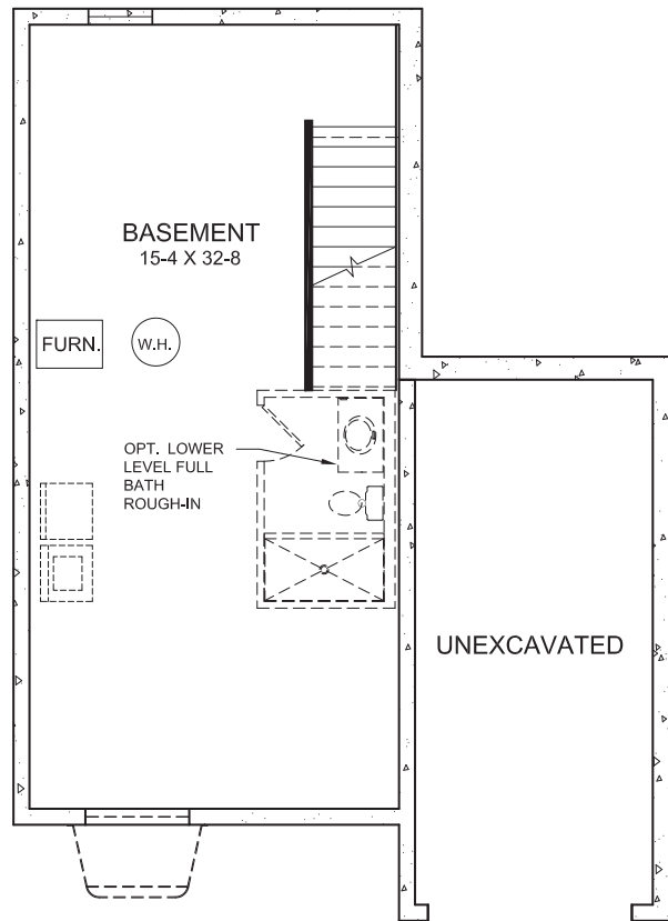
BASEMENT DESIGN A
