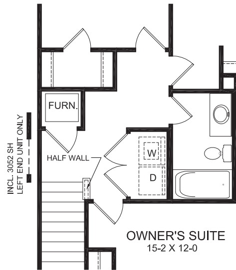
SECOND FLOOR DESIGN OPTIONAL STANDARD PLAN
