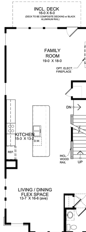
MAIN LEVEL DESIGN
