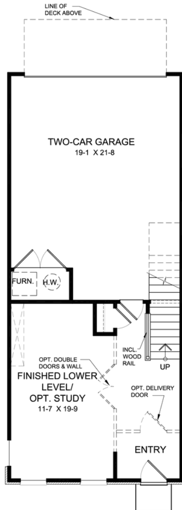
LOWER LEVEL DESIGN
